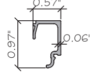
⑨ GLAZING CHANNEL YY86-47 6063-T5
