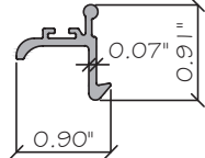
⑧ LOCK EXTRUSION YY86-46 6063-T5
