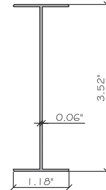
㉙ VERTICAL MULLION YY86-32 6063-T6
