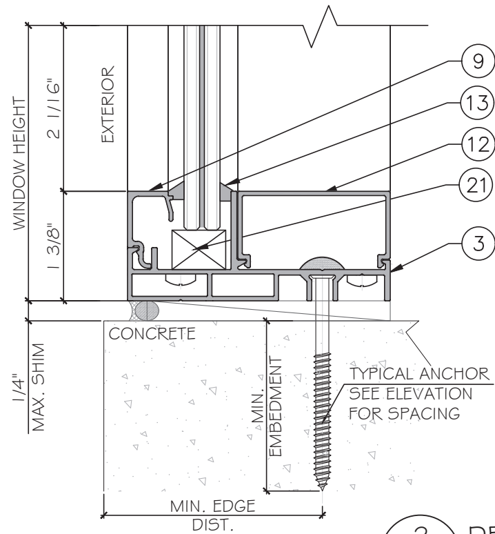
2 D4 DETAIL
